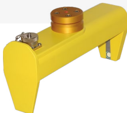
ROTARY SENSOR BF 600 C-E, BF 600 P-E > P/N 431 000 026
