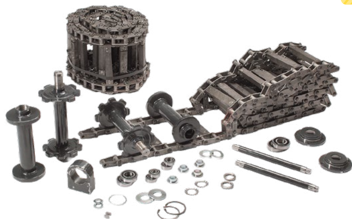
SLAT CONVEYOR CHAIN, KIT BF 300
